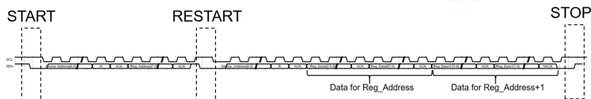
Figure 5-4 I 2 C Sequential Read with RESTART
