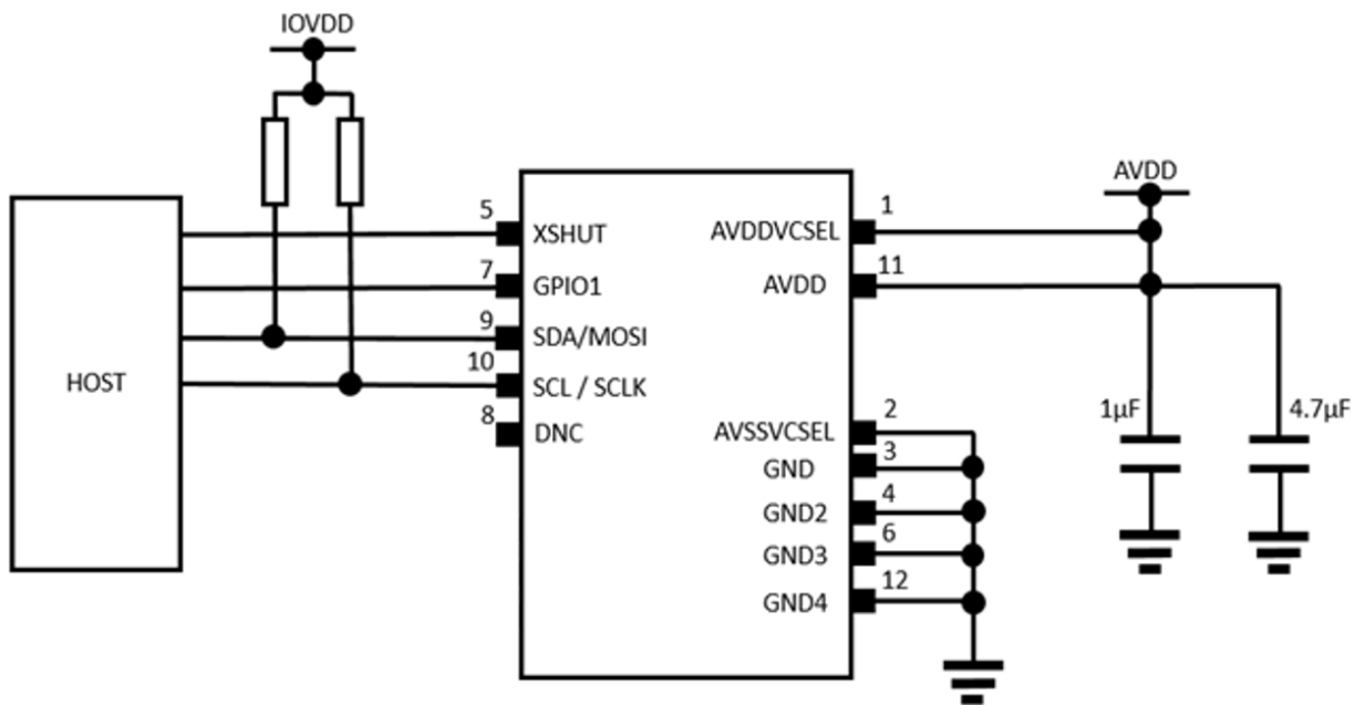
Figure 9-1 ADS6102 Application Schematic of I 2 C
