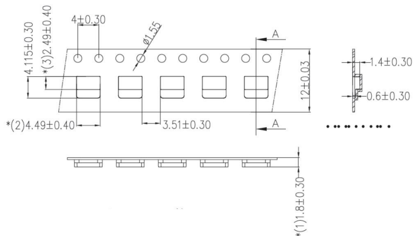
Figure 9-2 ADS6102 OLGA12 Tape and outline drawing
