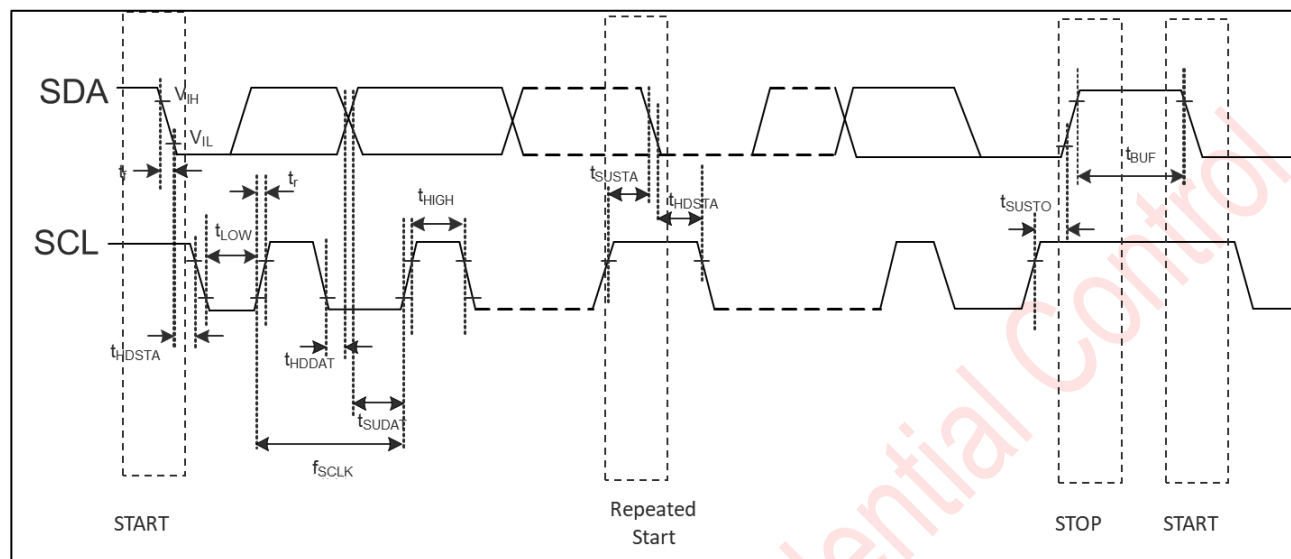
Figure 5-6 I 2 C Timing Specification
