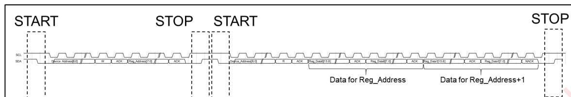
Figure 5-3 I 2 C Sequential Read with STOP / START
