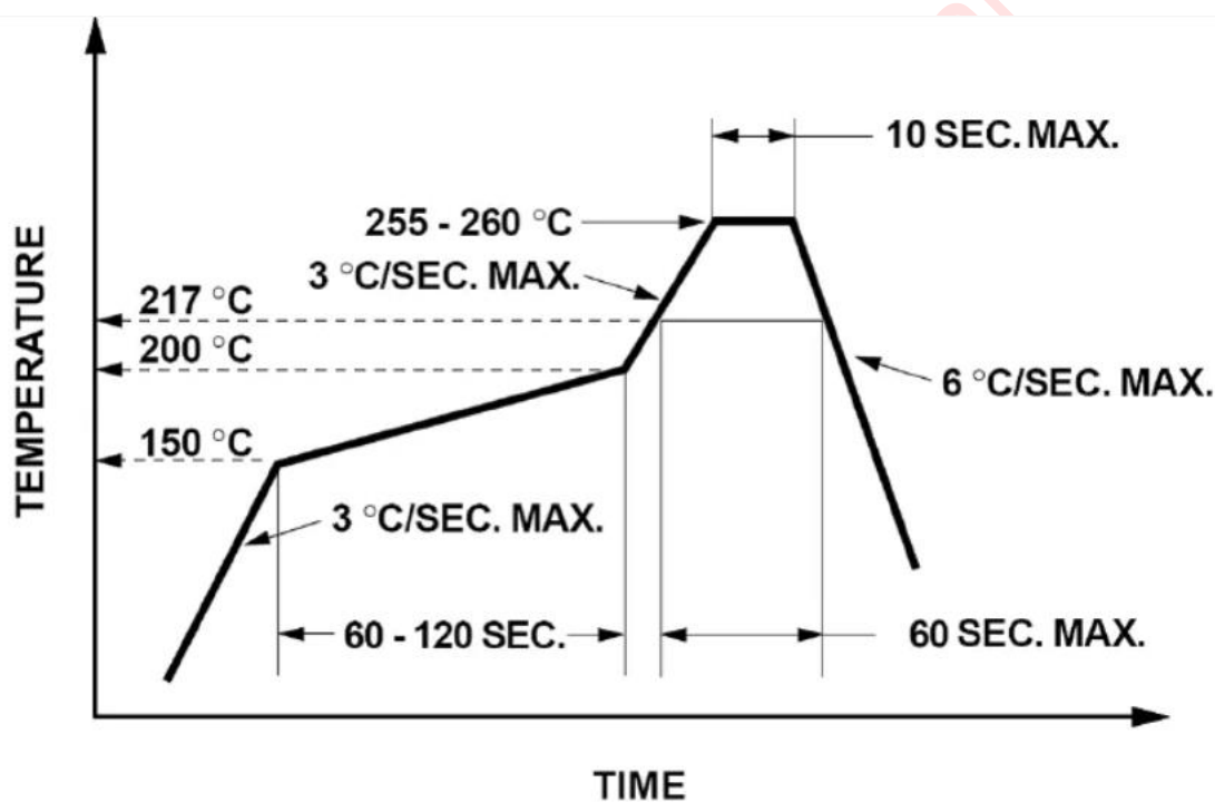
Figure 10-1 Reflow Soldering
