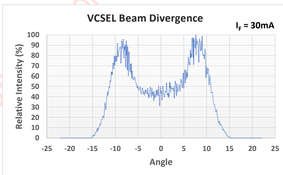
Figure 4-1-2 VCSEL Beam Divergence
