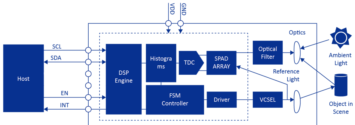
Figure 2-1 ADS6102 Block Diagram
