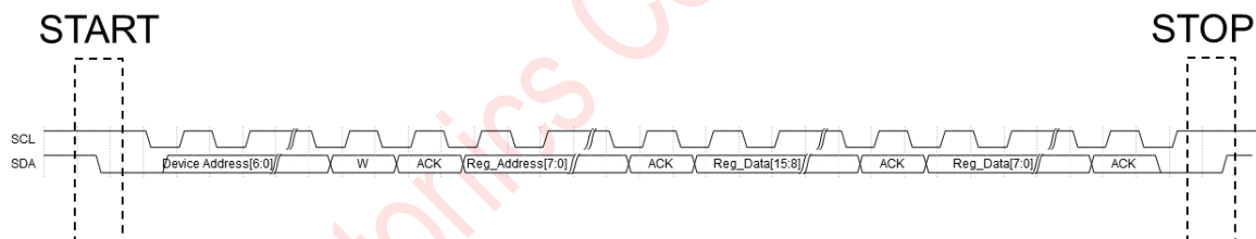
Figure 5-1 I 2 C Write
