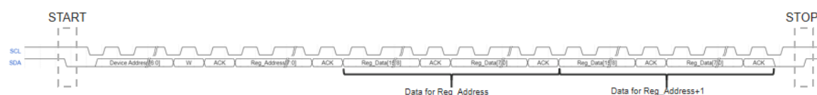
Figure 5-5 I 2 C Sequential Write
