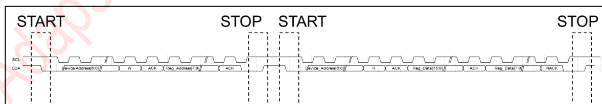
Figure 5-2 I 2 C Read
