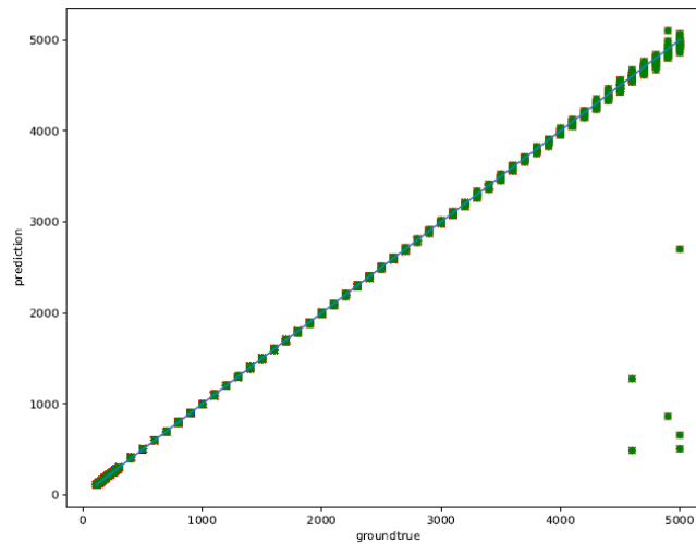
Figure 6-1 88 % White Card, ranging distance 110 mm to 5000 mm
