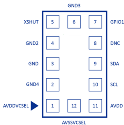
Figure 2-2 ADS6102 Pin Diagram (TOP VIEW)
