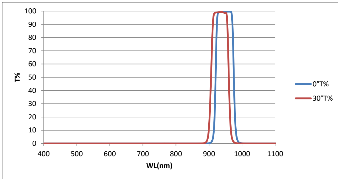
Figure 4-3-1 Cut Band (400 ~ 900 & 995 ~ 1100)
