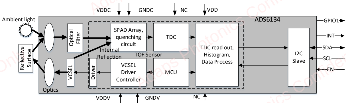
Figure 1-1 ADS6134 Block Diagram
