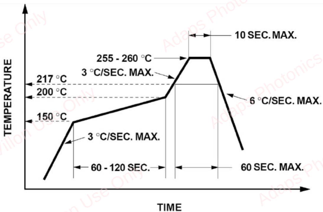
Figure 8-1 Reflow Soldering
