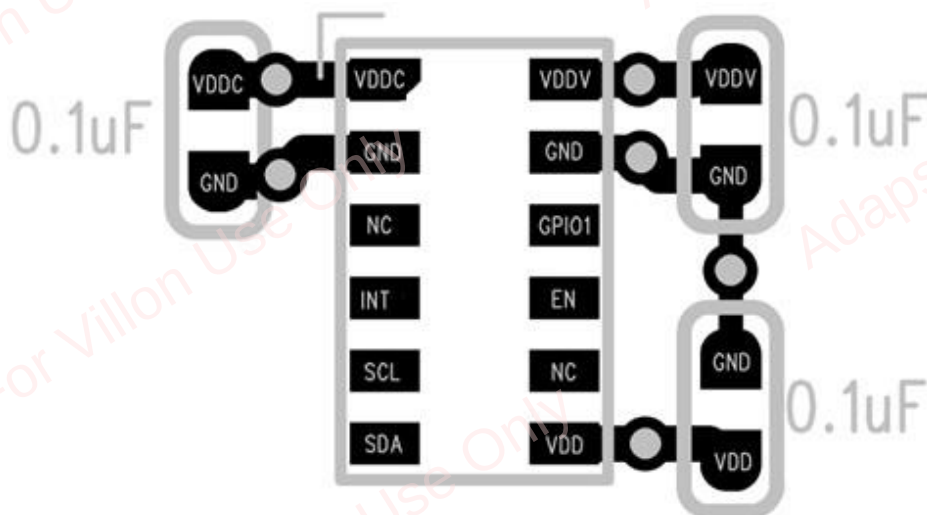
Figure 2-2 ADS6134 PCB Layout Recommendation
