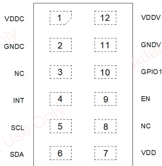
Figure 1-2 ADS6134 Pin Diagram (TOP VIEW)
