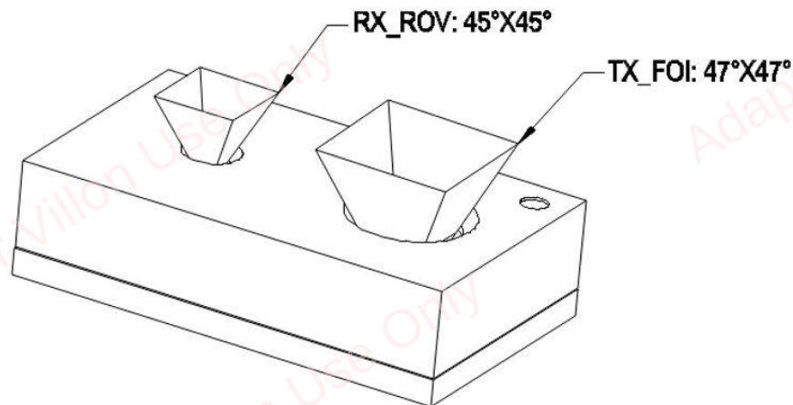
Figure 7-3 FoV/FoI Drawing
