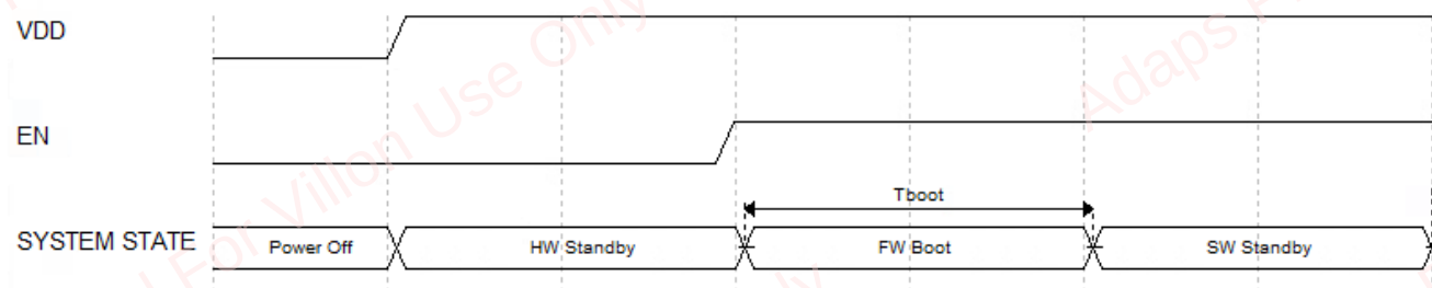
Figure 3-1 Power up and boot sequence (EN is controlled)
