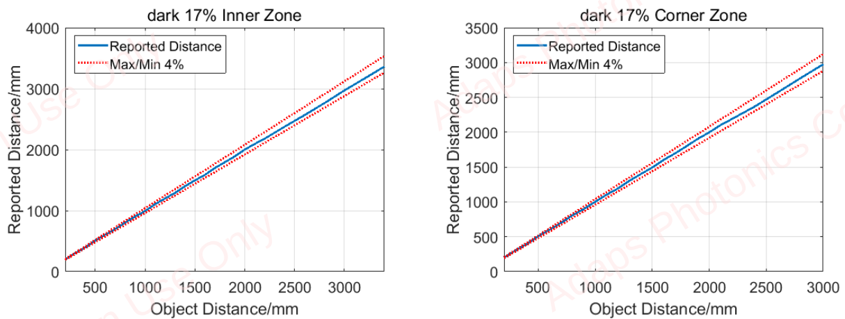
Figure 5-4 17 % Grey Card, inner and corner zone ranging performance
