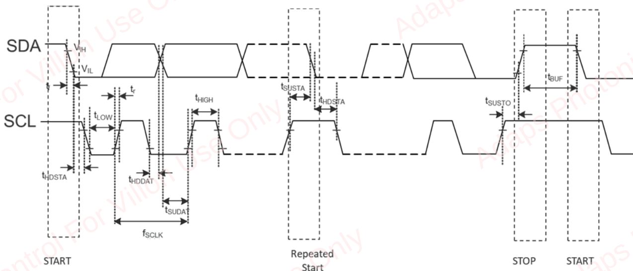
Figure 4-1 I 2 C Timing Specification
