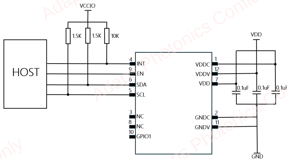
Figure 2-1 ADS6134 Application Schematic
