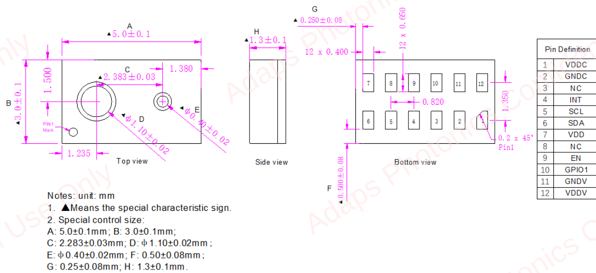
Figure 7-2 Package Outline Drawing
