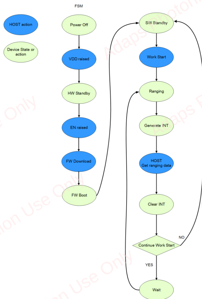
Figure 3-3 State Machine
