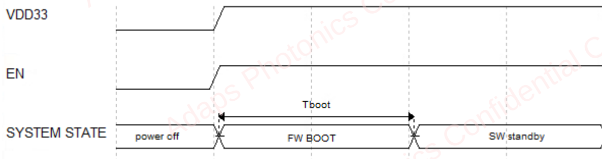
Figure 3-2 Power up and boot sequence (EN is not controlled)
