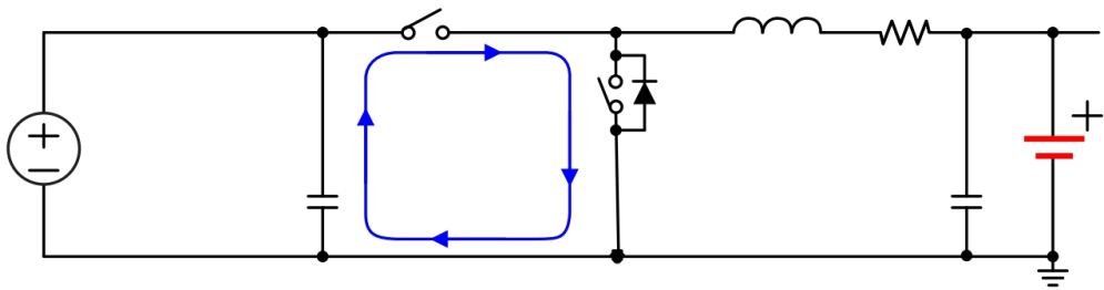
Figure 10-1. High Frequency Current Path
