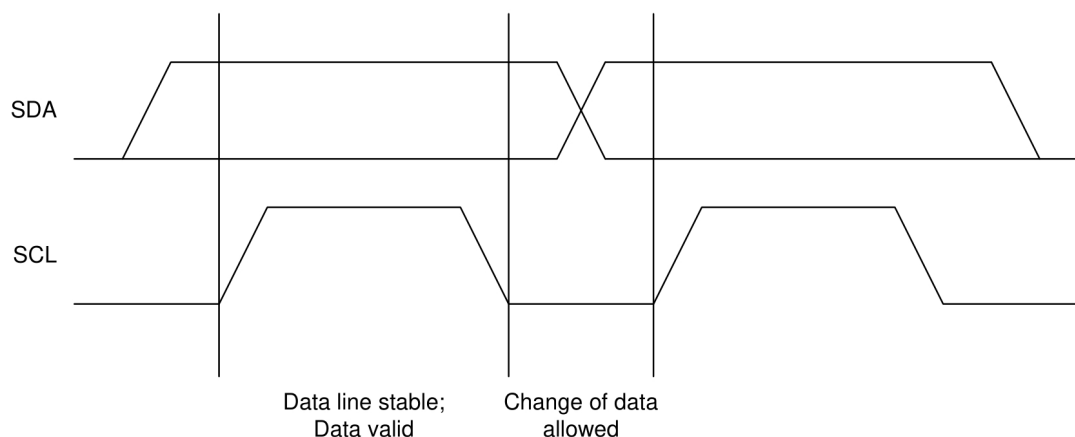
Figure 7-9. Bit Transfer on the I 2 C Bus
