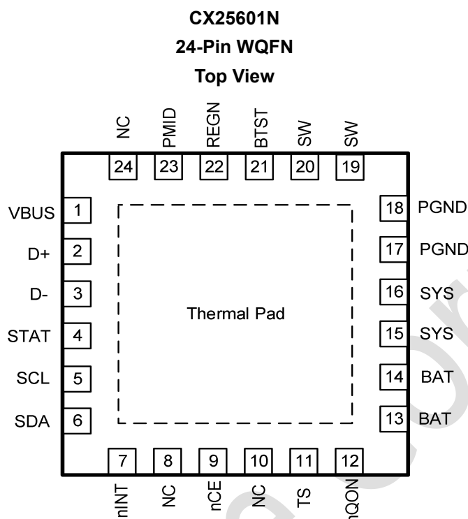
PIN Functions
