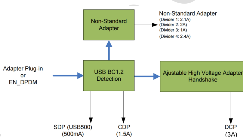
Figure 7-1. D+/D- Detection Flow
