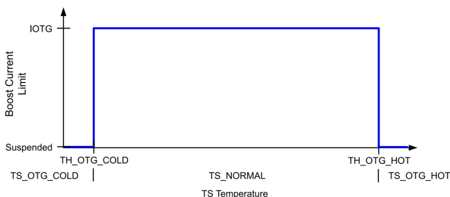
Figure 7-6. TS Pin Thermistor Sense Threshold in Boost Mode
