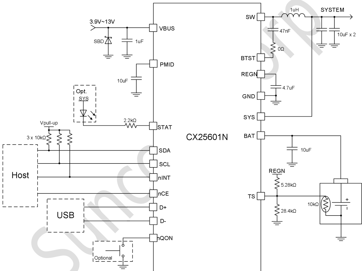
Figure 8-1. CX25601N Application Diagram
