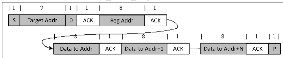
Figure 7-15. Multi-Write
