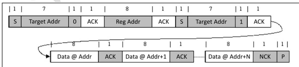
Figure 7-16. Multi-Read
