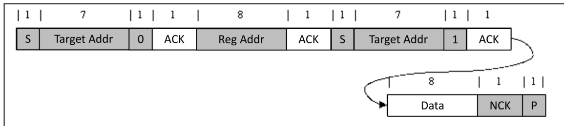
Figure 7-14. Single Read
