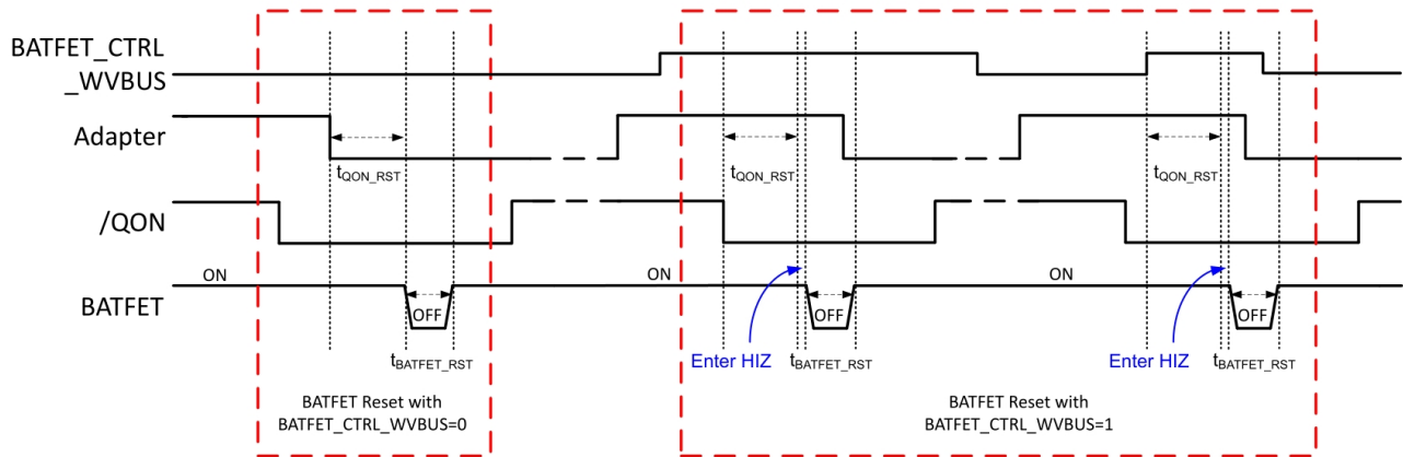
Figure 7-7. System Power Reset Timing
