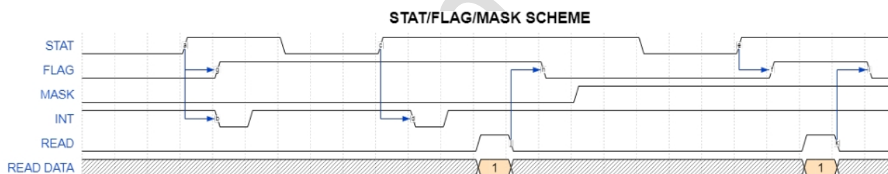
Figure 7-8. Relationship Between STAT, FLAG, and MASK
