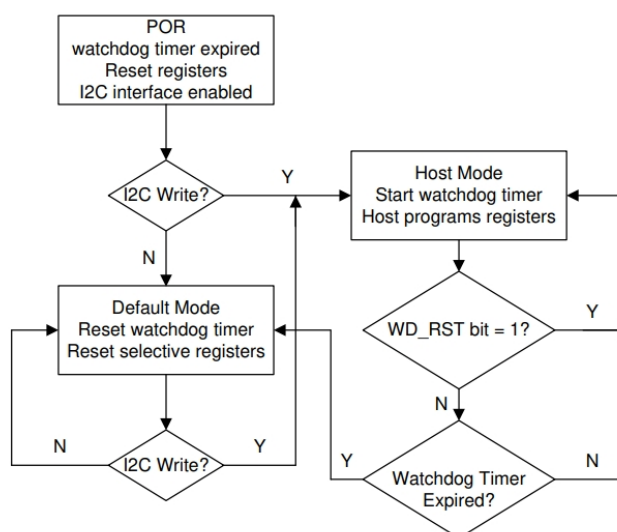
Figure 7-2. Watchdog Timer Flow Chart
