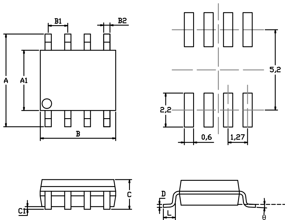
ESOP8 package mechanical data
