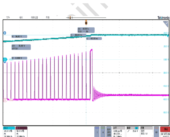
输出过压保护(OVP) CH2:Vout,CH3:Vsw
